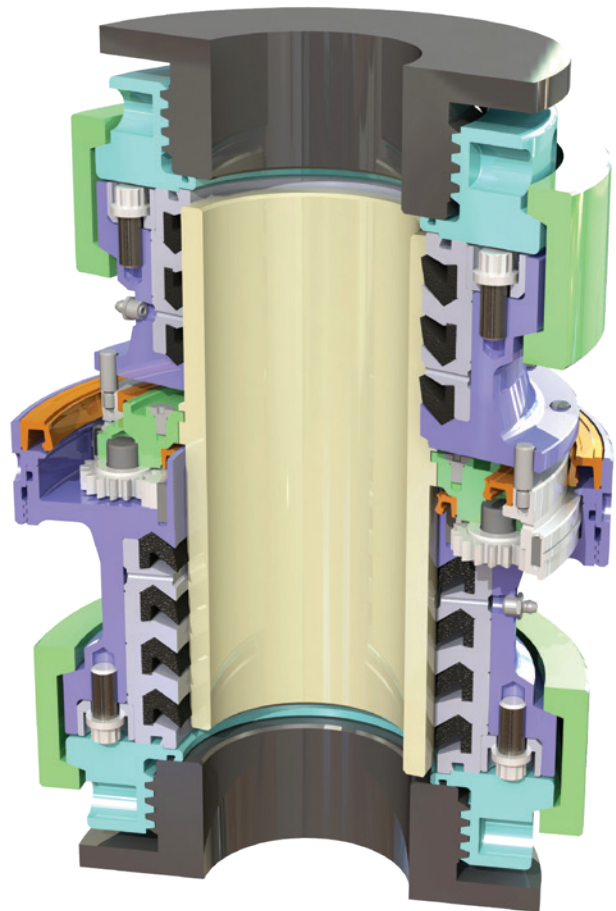
Sur-Drive™ Epicyclic Swivel Available in 3" and 4" ID Sizes Patent Pending
