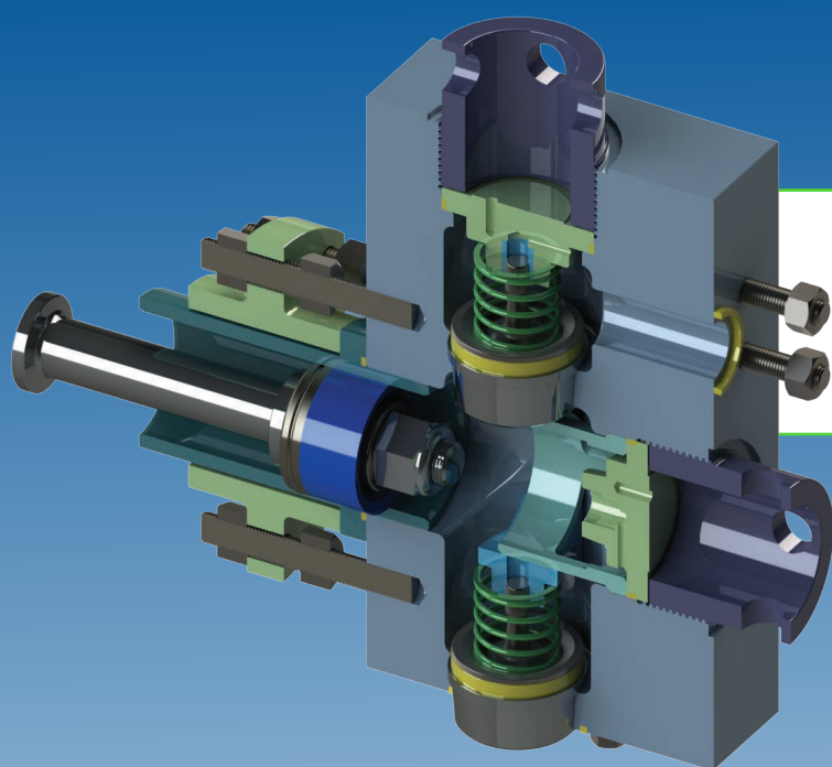
PAH Liner/Piston Arrangement
